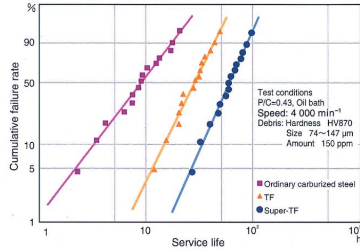
Fig. 10 Service life of L44649/10 bearings under contaminated lubrication
