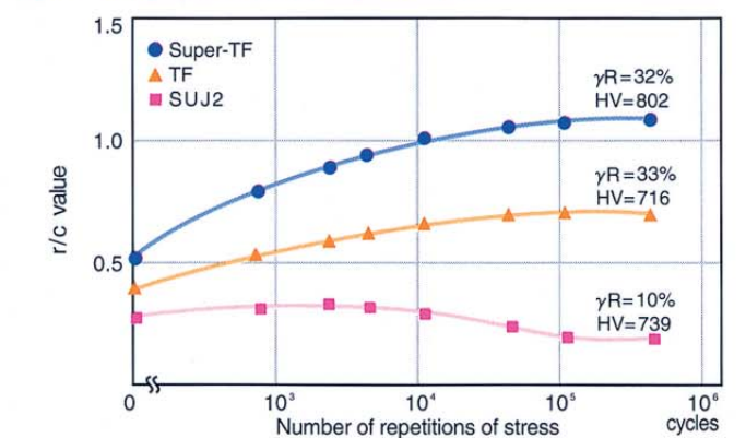
Fig. 9 Change of r/c value under repeated stress
