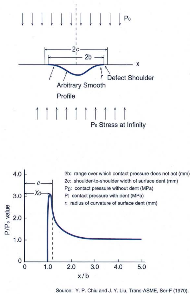
Fig. 2 Concentration of stress around a surface dent
