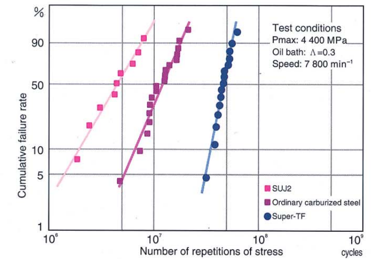
Fig. 13 Service life tests with boundary lubrication
