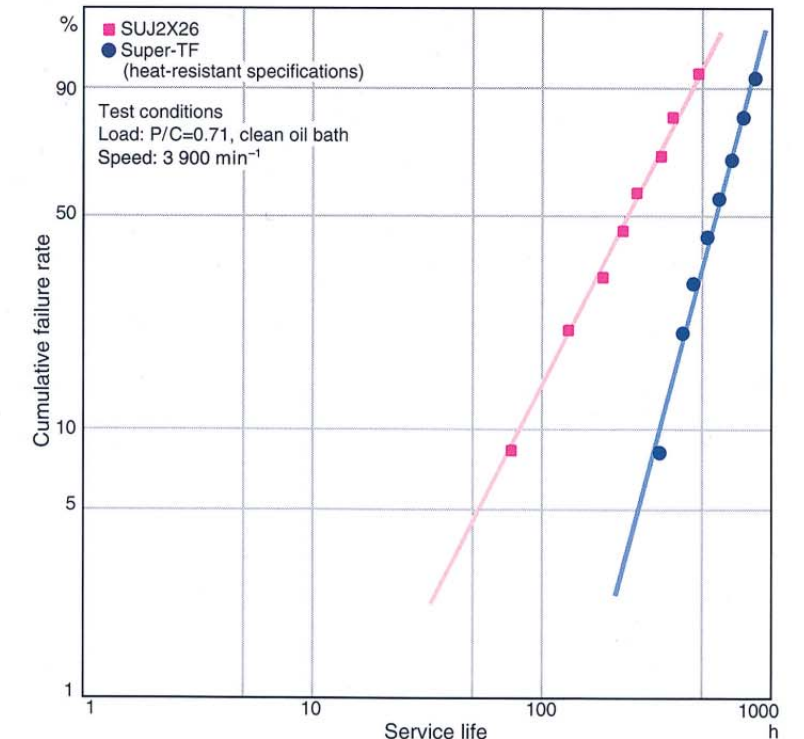
Fig. 15 Service life of 6206 ball bearings at 160°C under clean lubrication
