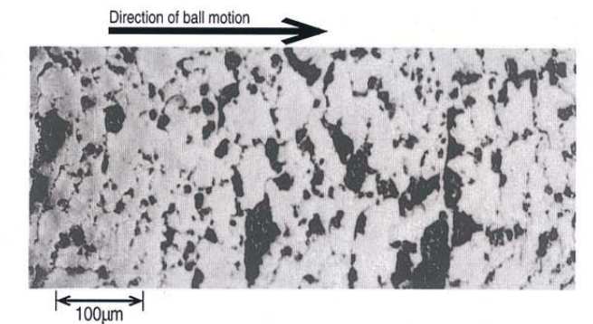
Fig. 14 Peeling damage
