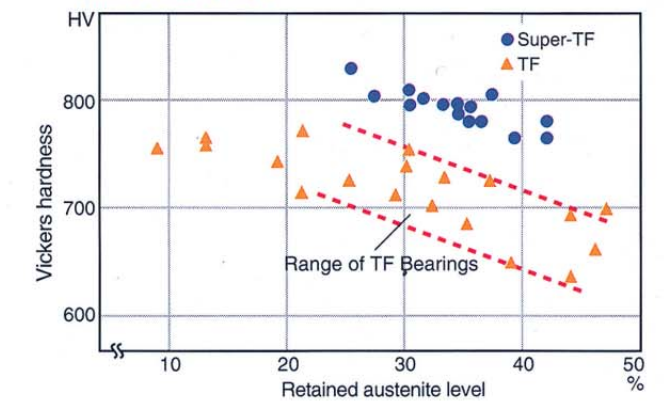
Fig. 8 Relationship of material hardness and retained austenite level
