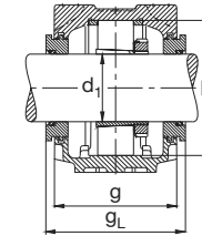
Anel labirinto TSV
