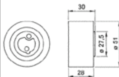
VKM 76001
