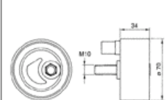
VKM 78000
