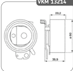
VKM 13214
